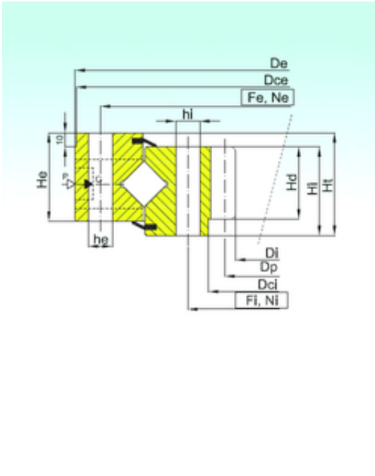
ZR1.25.0946.400-1SPPN Bearing 2D drawings and 3D CAD models
