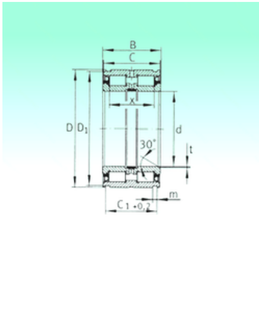
SL045006-PP Bearing 2D drawings and 3D CAD models
